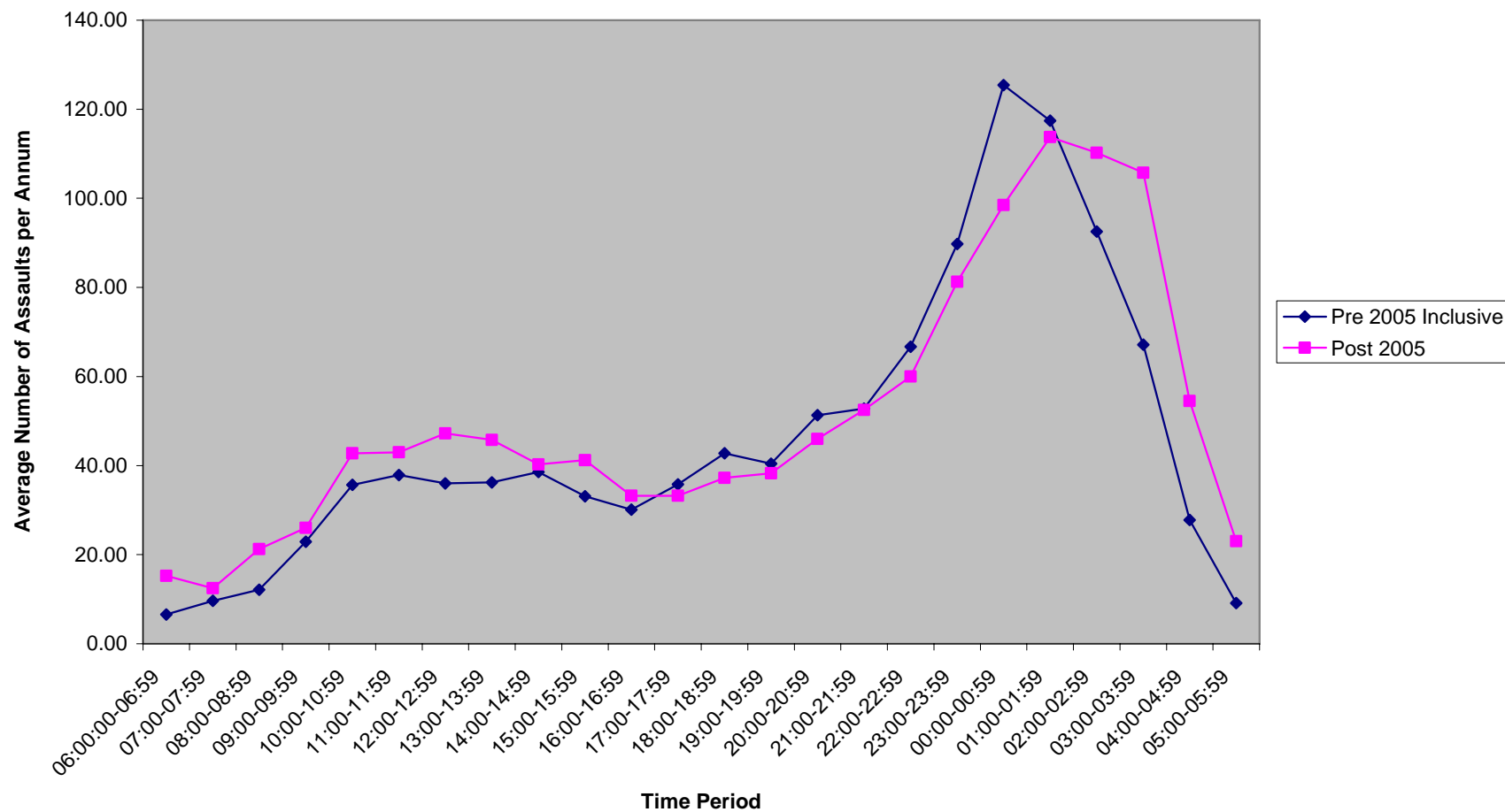
Average Numbers of Assaults per Year Presenting Pre/Post 2005 in Different Time Periods
